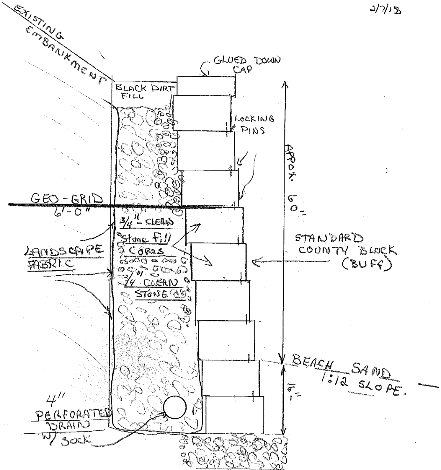
CROSS SECTION OF TALLEST WALL Scale 1" = 1'
